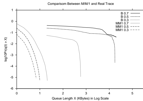
Figure 5: Queueing experiment for M/M/1 model and the LRD All1 trace.
