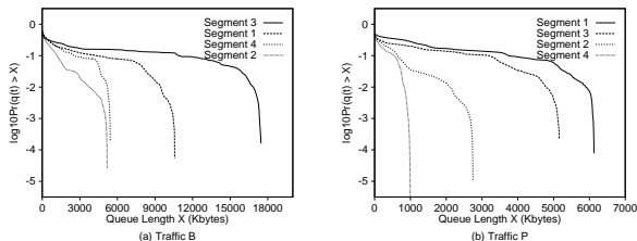
Figure 7: Queueing experiment of Segments from trace All7 with 0.7 utilization.
