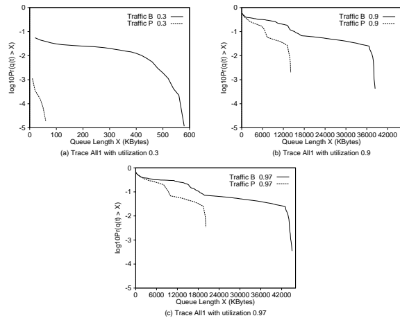
Figure 9: Queueing experiments for trace All1 with 0.3, 0.9 and 0.97 utilizations.
