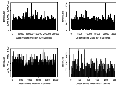
Figure 2: Bursty Traffic Over Many Time Scales.
