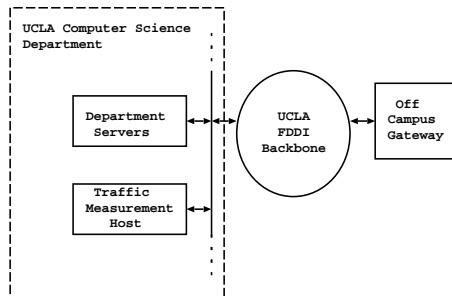
Figure 1: UCLA CSD Measurement Connection.
