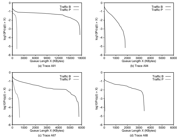
Figure 8: Queueing experiment of each trace with 0.5 utilization.
