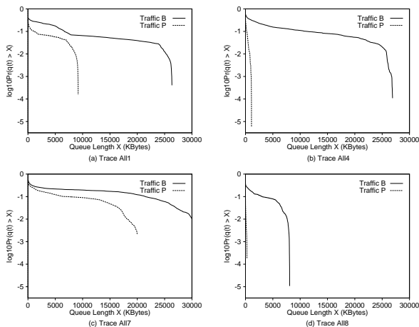
Figure 6: Queueing experiment of each trace with 0.7 utilization.
