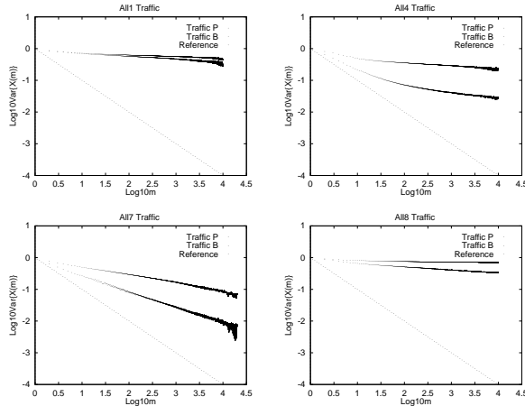
Figure 4: Variance-time plots for the 4 traces.
