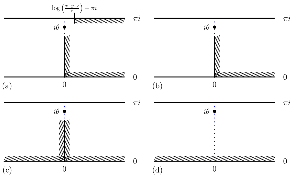
Figure 6: (a) The image of the domain \mathbb{H} \setminus A_{R,r} and the point z under the map w \mapsto \log\left(\frac{w-x}{r}\right) . The point z goes to i\theta , from which we measure all the harmonic measure terms. The tick marks highlight the boundary segment referred to as V_2 . (b) Removing some of the tick marks from (a) only makes the harmonic measure smaller. (c) By symmetry, the harmonic measure in (c) is twice the harmonic measure in (b). (d) Removing the slit from (c) only decreases the harmonic measure.
