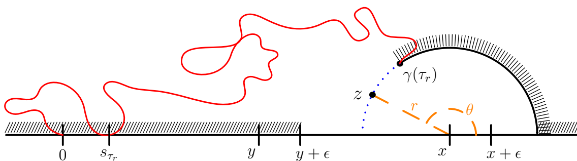
Figure 5: The domain \mathbb{H} \setminus A_{R,r} indicated by solid black boundaries, with the curve \gamma([0, \tau_r]) sitting inside it. The boundary segment V_1 is highlighted by tick marks. Any Brownian path started at z that exits \mathbb{H} \setminus A_{R,r} on V_1 is also a Brownian path in \mathbb{H} \setminus K_{\tau_r} that exits \mathbb{H} \setminus K_{\tau_r} on [s_{\tau_r}, y + \epsilon] or the right side of K_{\tau_r} .
